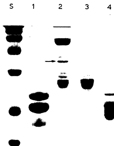
Fig.2. Gel electrophoresis of the fractionated caiman crystallins under denaturing conditions (SDS-PAGE) in the presence of 5 mM dithiothreitol. Lane S, standard proteins used as molecular mass markers (in kDa): transferrein (80), bovine serum albumin (66), ovalbumin (45), carbonic anhydrase (30), soybean trypsin inhibitor (20.1) and lysozyme (14.5). Lanes 1–4 correspond to the 4 fractions (Cm-1–Cm-4) of fig.1A. The gel was stained with Coomassie blue. The arrow in lane 2 indicates the minor \epsilon -crystallin subunit of 37.5 kDa.
